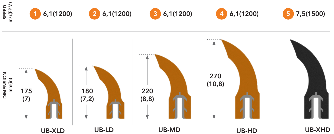
Figure 1. Maximum speed according to type of primary urethane belt cleaner m/s (FPM)
